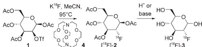
Scheme 1. Conventional radiosynthesis of ^{18}\text{F} FDG ( ^{18}\text{F} -3). Tf = triflate.
