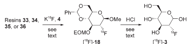
Scheme 7. Synthesis of [\text{F}^{18}]\text{FDG} from resin-bound precursors.
